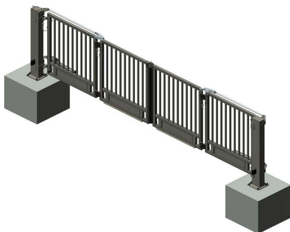
Double-leaf (four segments) with drive unit and deflection system Maximum opening width 6 m Solid posts 250 x 150 mm with integrated control
